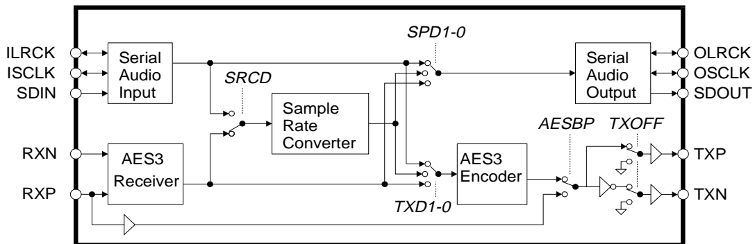
Figure 2. Software Mode Audio Data Flow Switching Options
