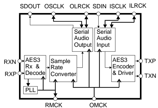
Figure 6. Serial Audio Input, AES3 Input Clock Source, SRC Enabled
