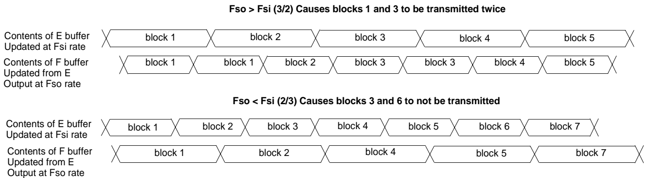
Figure 36. Channel Status Block Handling When Fso is Not Equal to Fsi
