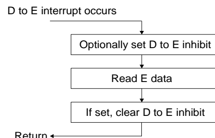
Figure 37. Flowchart for Reading the E Buffer
