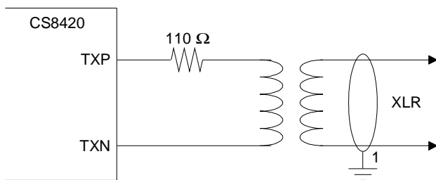
Figure 28. Professional Output Circuit
