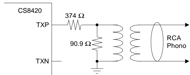
Figure 29. Consumer Output Circuit
