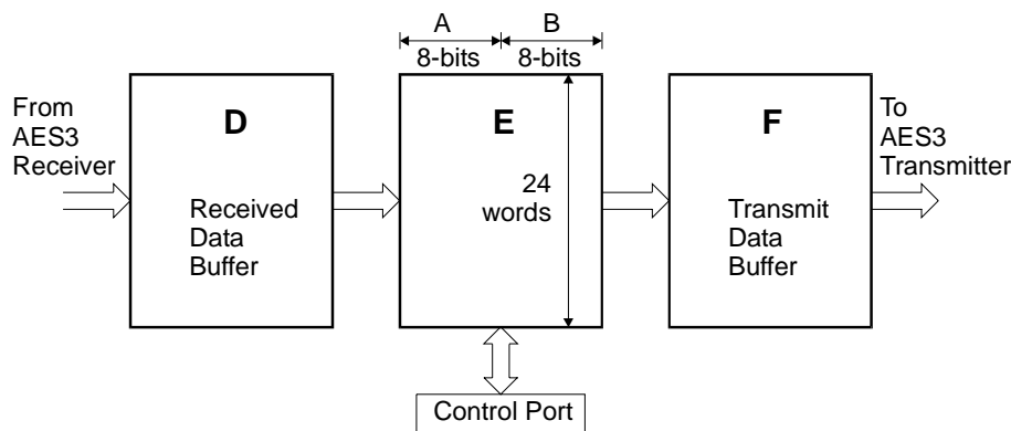
Figure 35. Channel Status Data Buffer Structure
