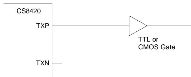
Figure 30. TTL/CMOS Output Circuit
