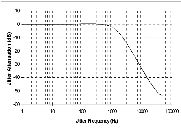
Figure 14. Jitter Attenuation Characteristics of PLL with “slow” Filter Components
