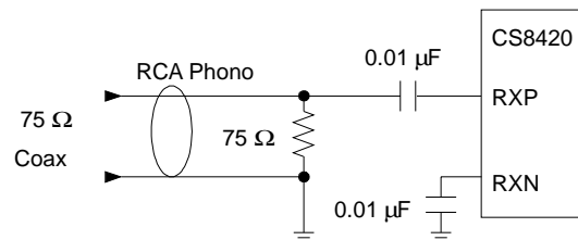
Figure 33. Consumer Input Circuit
