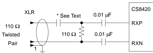
Figure 32. Transformerless Professional Input Circuit
